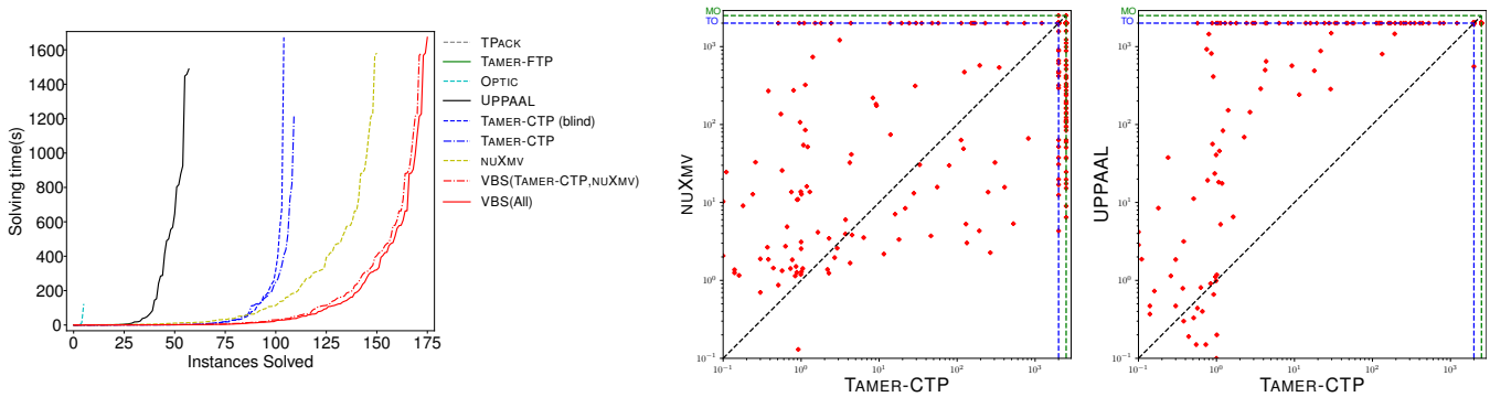
Figure 2: (Above) Coverage table showing results for solvable and unsolvable benchmarks. (Below) Plots for the unsolvable benchmarks: cactus plot (left) and scatter plots comparing TAMER-CTP with NUXMV (center) and UPPAAL (right).
