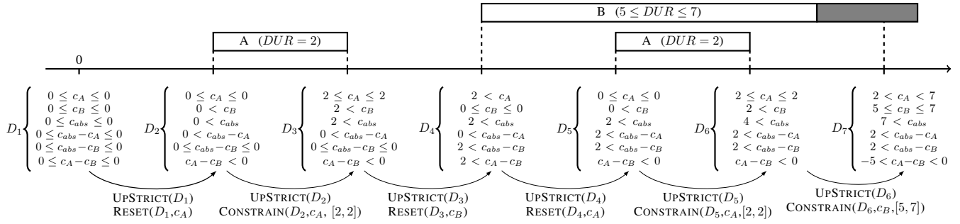
Figure 1: Example of DBM usage in TAMER-CTP. The temporal constraints in the example plan depicted as a Gantt chart are captured by the sequence of DBM constraints on the clocks c_{abs} (the absolute clock, i.e. the time since the plan has started), c_a and c_b .
